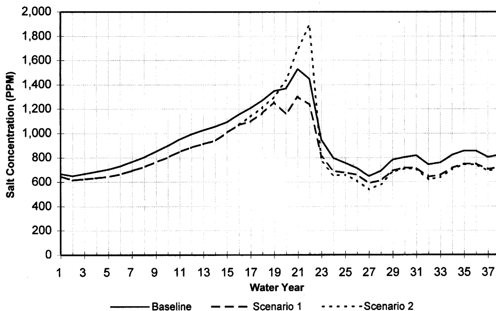
Figure 6. Salt Concentration Below Lake Mead Under the Baseline, Scenario 1, and Scenario 2, with SSD Inflow Hydrology.
