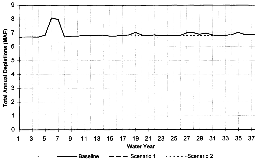
Figure 5. Lower Basin Total Annual Depletions Under the Baseline, Scenario 1, and Scenario 2, with SSD Inflow Hydrology.
