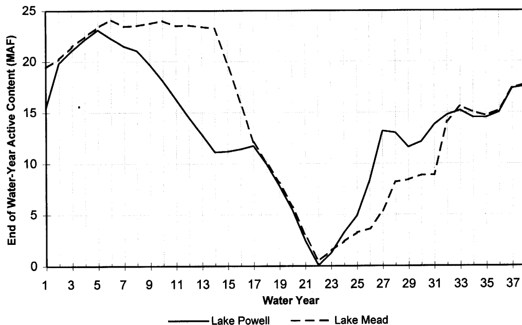
Figure 9. Lake Powell and Lake Mead End of Water-Year Active Content Under Scenario 2 (CRC Call Suspended), with SSD Inflow Hydrology.
