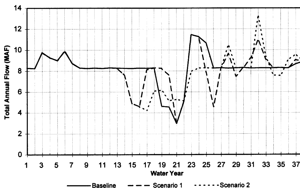
Figure 2. Total Annual Flow at Lee Ferry Under the Baseline, Scenario 1, and Scenario 2, with SSD Inflow Hydrology.
