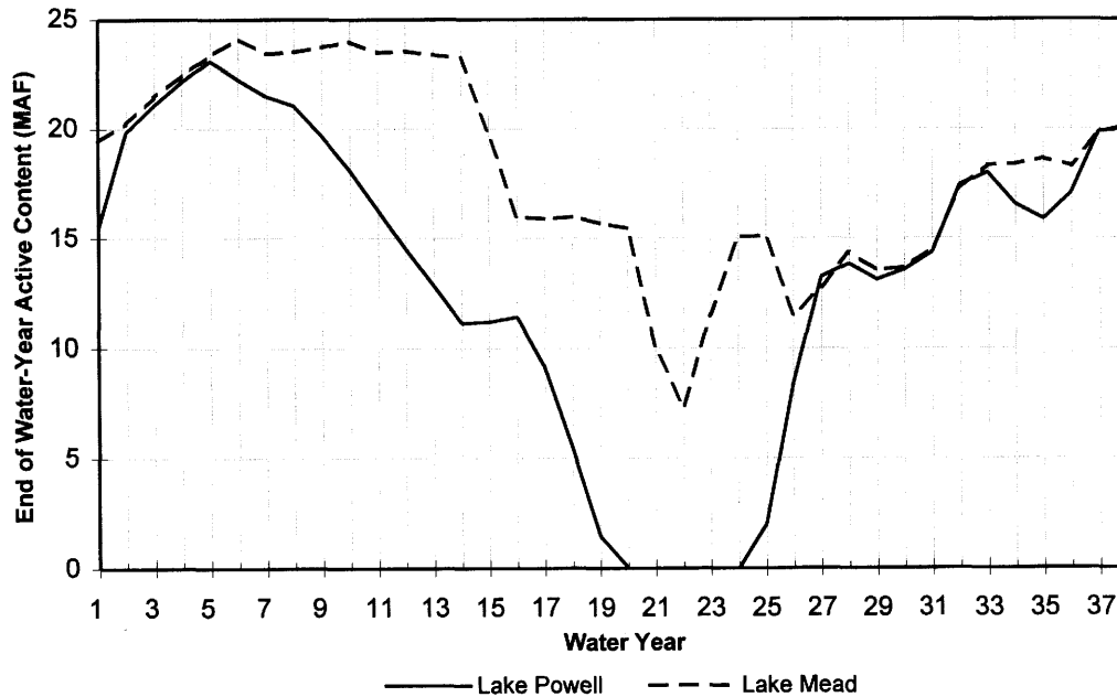
Figure 8. Lake Powell and Lake Mead End of Water-Year Active Content Under Scenario 1 (CRC Call Enforced), with SSD Inflow Hydrology.
