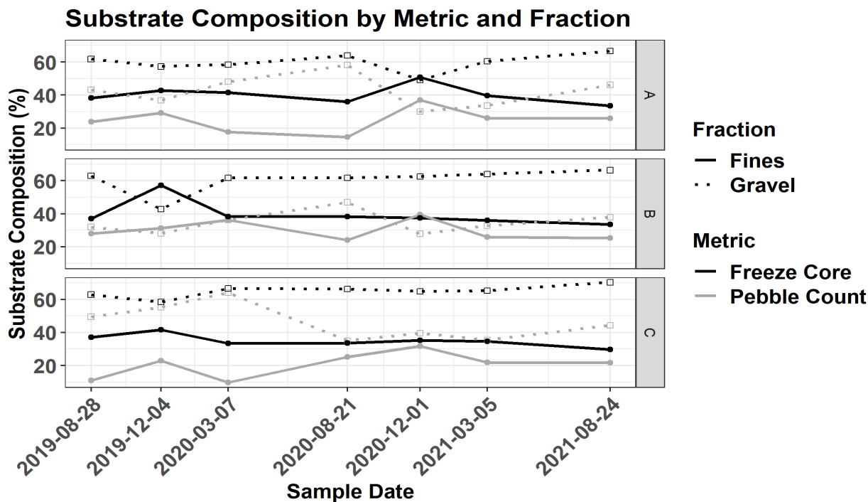
Figure 2. Temporal trends in the size composition of surface (pebble counts, grey) and subsurface (freeze cores, black) spawning habitat as represented by the percentages of fine sediment (<2 mm in diameter, solid line) and gravel (2 – 64 mm, dashed line) of streambed substrate at three sampling sites. An increase in the percent fine material (<2 mm) was observed during the post drawdown sampling events (December) across all sites, but more pronounced at Site A. The proportion of fines in the streambed surface and substrate composition was similar for both sample metrics although the magnitudes differed with pebble counts indicating a lesser percentage of the substrate composition being derived from fine material (<2 mm).
