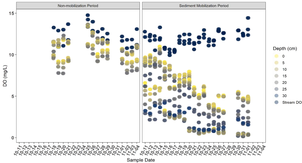
Figure 7. Average hyporheic dissolved oxygen (mg/L) observed in standpipes (n = 5/site) during non-sediment mobilization experimental CSFOs (fall 2020) and sediment mobilization experimental CSFOs (fall 2019 drawdown) averaged across. Color represents the hyporheic depth below the streambed surface (surface = yellow to 30 cm = dark blue) with stream dissolved oxygen represented in the darkest color.
