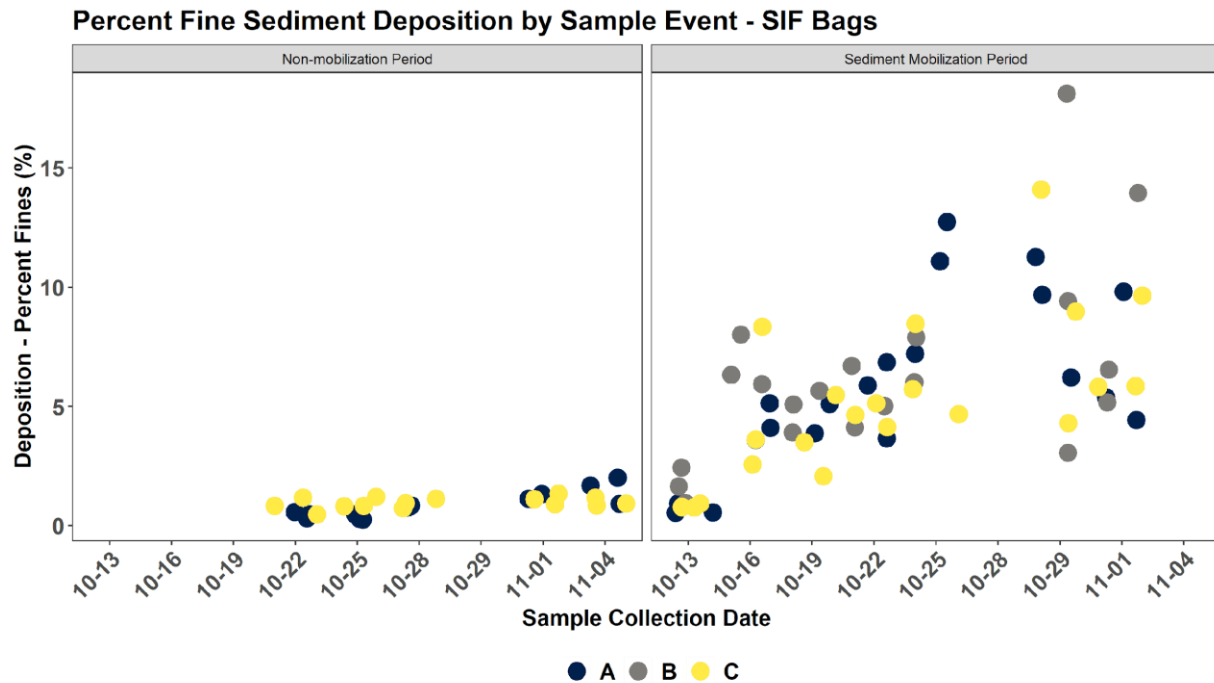
Figure 6. Average percent fine material (<2 mm) deposited in sediment infiltration bag samples by site (n = 3/site). Colors represent site as follows: blue = Site A, grey = Site B, yellow = Site C. Panels reflect non-sediment mobilization experiment CSFOs (left, 2020 fall drawdown period) and sediment mobilization experimental CSFOs (right, 2019 fall drawdown period).
