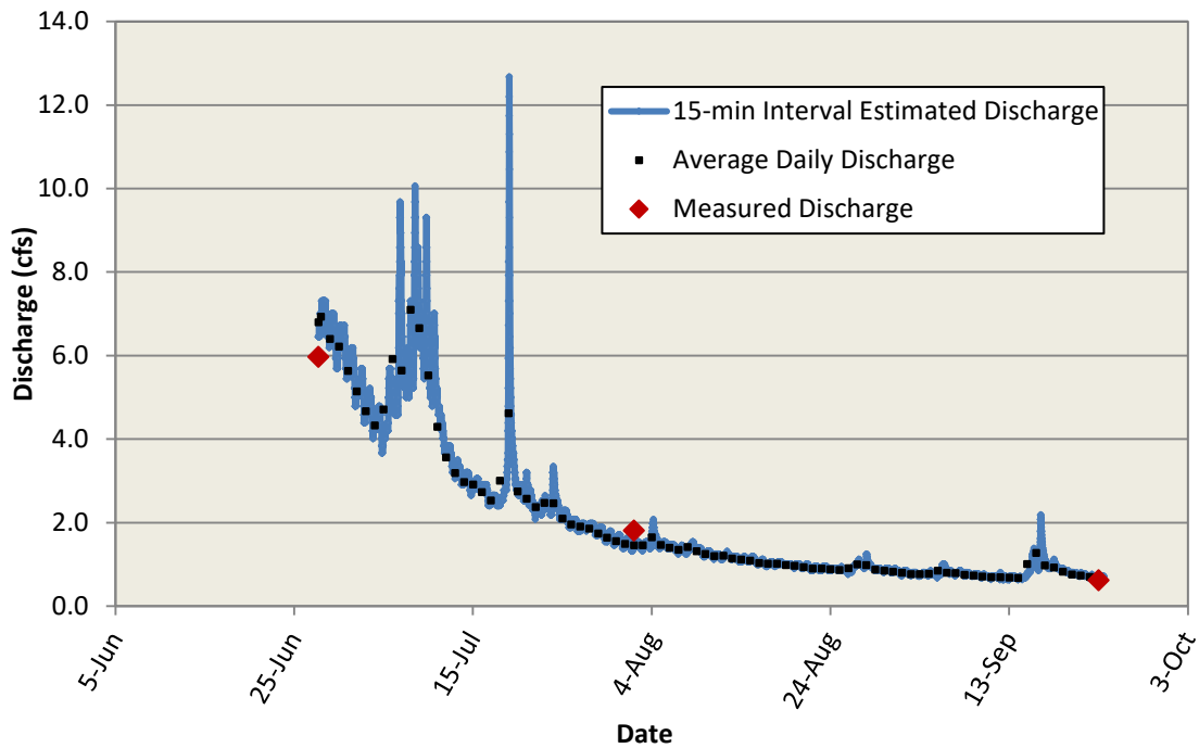
FIGURE 9. Estimated hydrograph for Middle Fork Long Creek study site during 2015.
