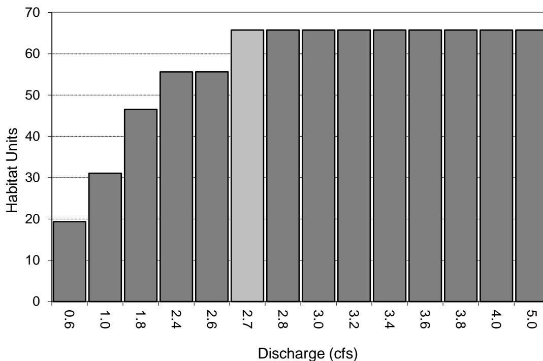
FIGURE 11. Habitat Quality Index vs. discharge in the Middle Fork Long Creek instream flow segment. X-axis values are not to scale; the values were chosen to indicate where changes in Habitat Units occur. The recommended flow (2.7 cfs) is needed to maintain the existing fishery and is indicated by the light shaded bar.
