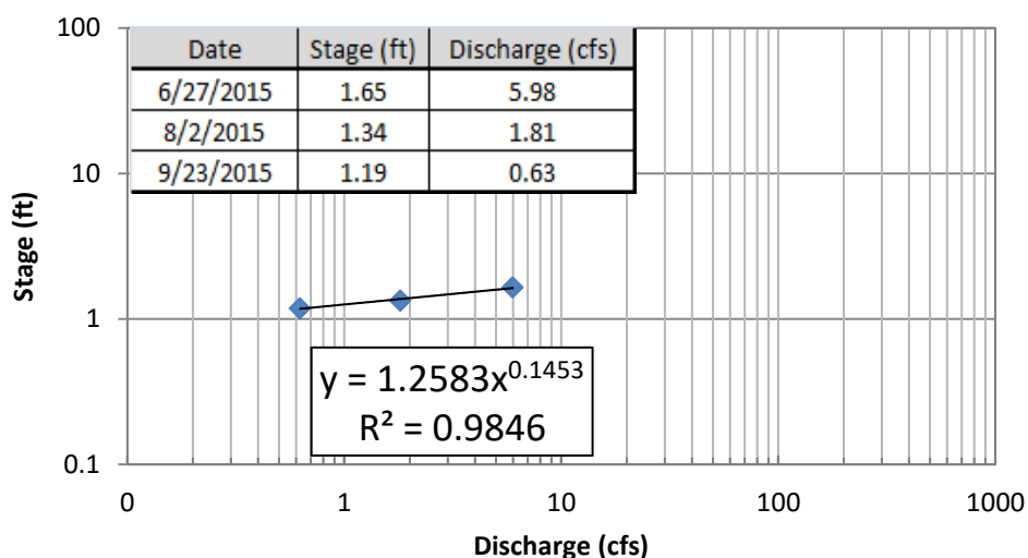
FIGURE 8. Rating curve data for the temporary gage established at the Middle Fork Long Creek study site during 2015.
