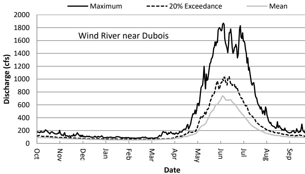
FIGURE 5. Hydrograph showing the maximum, 20% exceedance, and mean daily discharge for each day over a 64 year period of record (water years 1946-1992 and 2002-2018) at the Wind River near Dubois (USGS Gage 06218500) reference stream gage.
