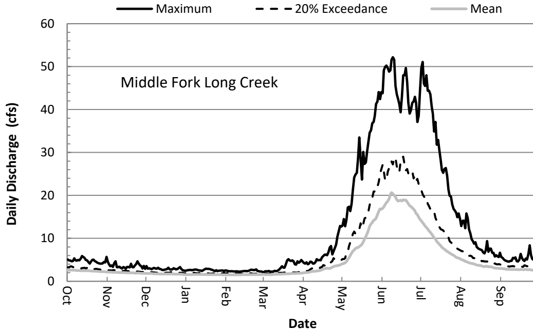
FIGURE C-4. Hydrograph showing the maximum, 20% exceedance, and mean daily discharge estimates for the Middle Fork Long Creek study segment.
