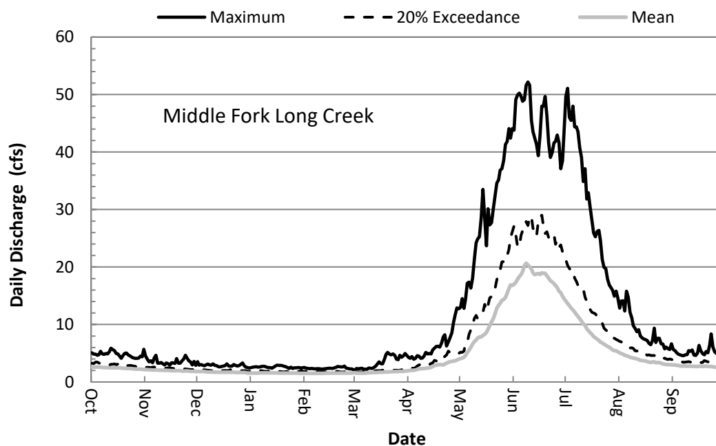
FIGURE 7. Hydrograph showing the maximum, 20% exceedance, and mean daily discharge estimates for the Middle Fork Long Creek study site.
