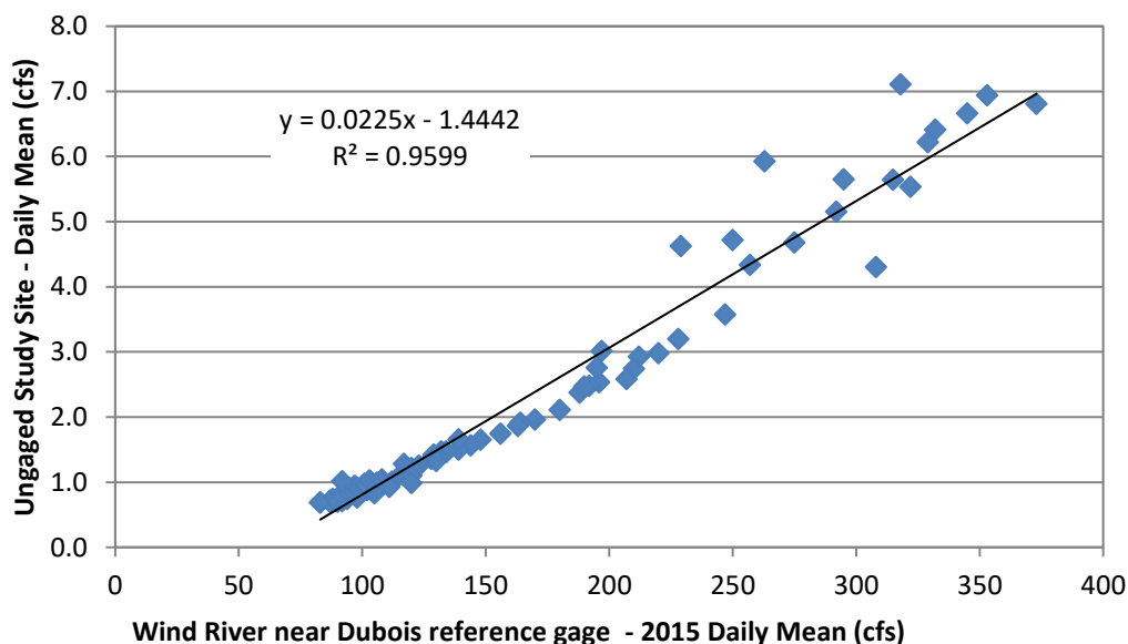
Figure C-3. Correlation between daily discharge estimates at the Middle Fork Long Creek study site in 2015 and the daily discharge estimates at the Wind River near Dubois (USGS Gage 06218500) reference gage.
