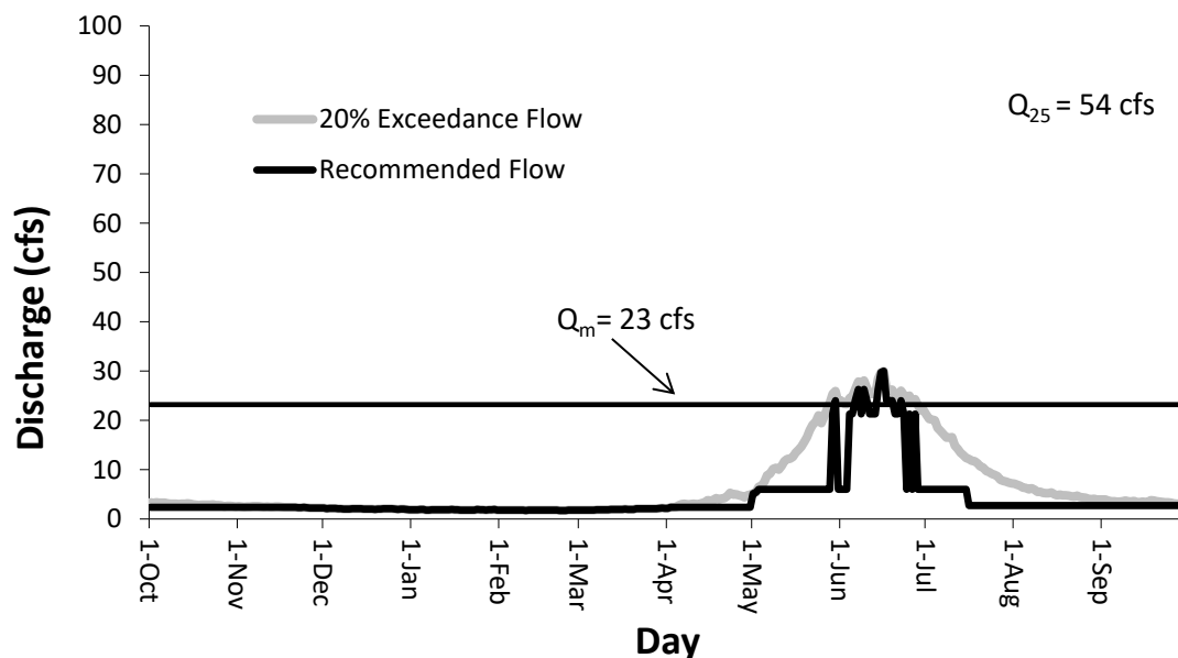
FIGURE B-3. Channel maintenance flow recommendations and hydrographs for the Middle Fork Long Creek instream flow segment if the flow were at the 20% exceedance flow all year.
