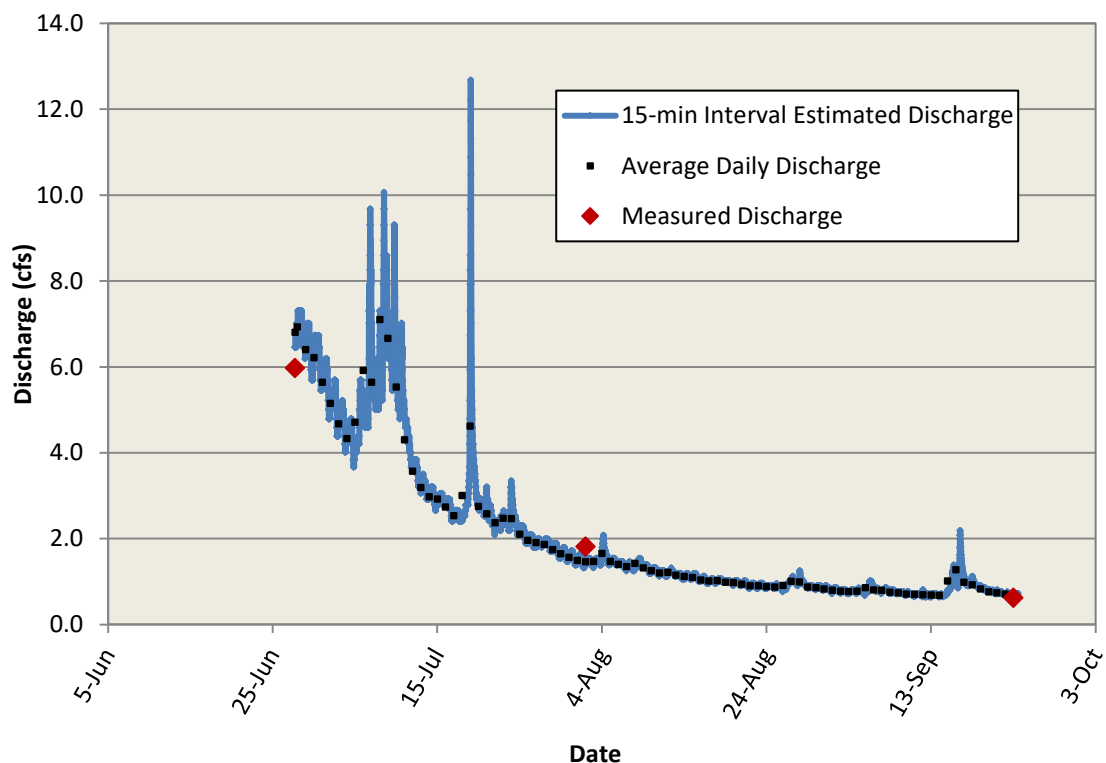
FIGURE C-2. Estimated hydrograph for Middle Fork Long Creek study site during 2015.
