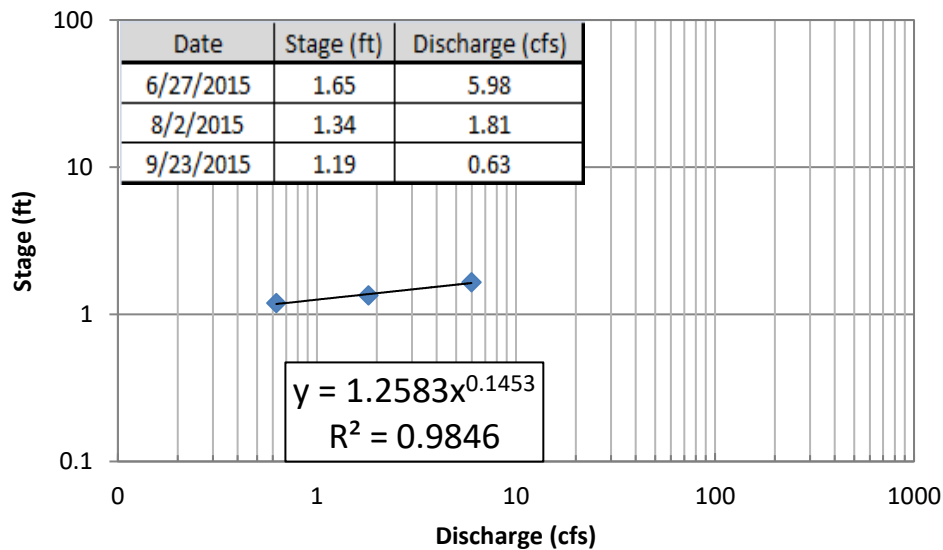
FIGURE C-1. Rating curve data for the temporary gage established at the Middle Fork Long Creek study site during 2015.
