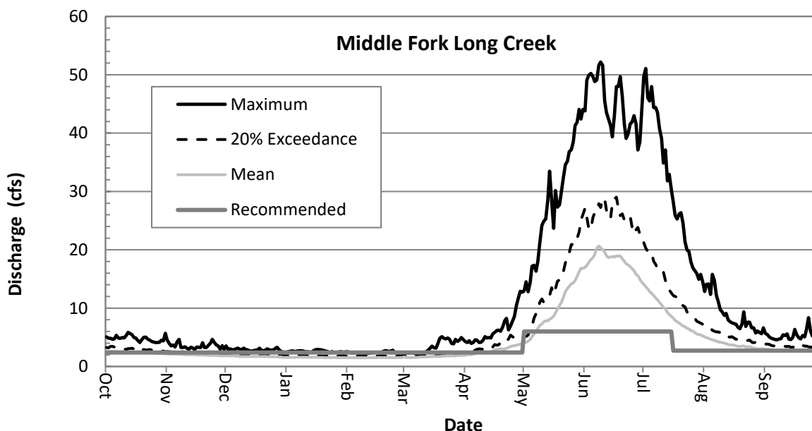
FIGURE 12. Recommended instream flow water right (when flows are naturally available) in the proposed segment relative to maximum, 20% exceedance, and mean daily discharge estimates.
