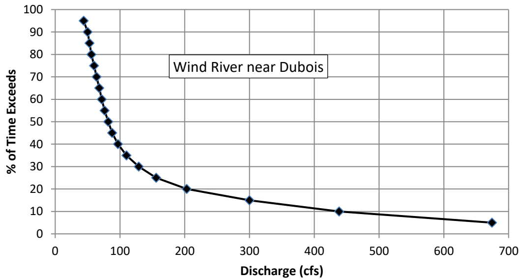
FIGURE 4. Flow exceedance curve for the Wind River near Dubois (USGS Gage 06218500) over a 64 year period of record (water years 1946-1992 and 2002-2018).
