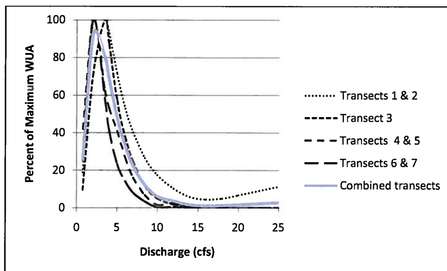
FIGURE 19. Weighted usable area available for CRC spawning at three study sites in Little Muddy Creek over a range of flows.
