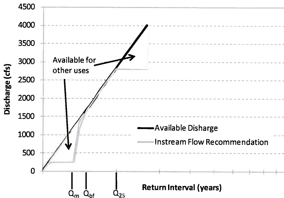
FIGURE A-2. General function of a dynamic hydrograph instream flow for fishery maintenance. Q_m is substrate mobilization flow, Q_{bf} is bankfull flow, and Q_{25} is the discharge with a 25-year return interval.
