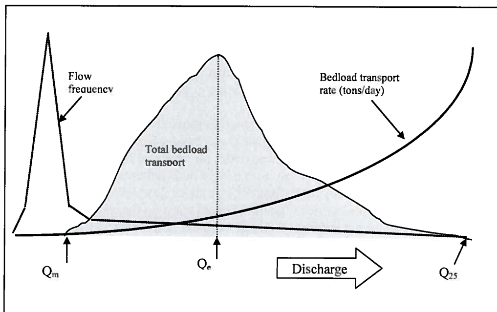
FIGURE A-1. Total bedload transport as a function of bedload transport rate and flow frequency (adapted from Schmidt and Potyondy 2004).
