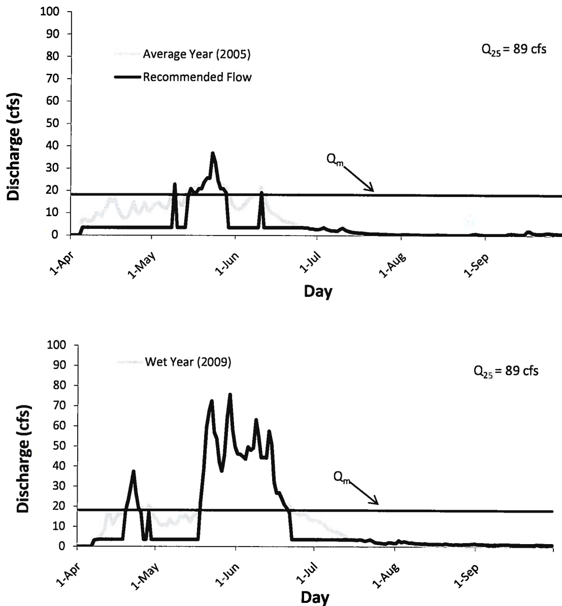
FIGURE A-3. Channel maintenance flow recommendations and hydrographs for the Muddy Creek instream flow segment in an average (2005) and a wet (2009) water year.
