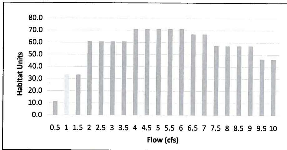
FIGURE 14. Habitat Quality Index vs. discharge in the Littlefield Creek instream flow segment. The recommended flow (1.0 cfs) is indicated by the light shaded bar.
