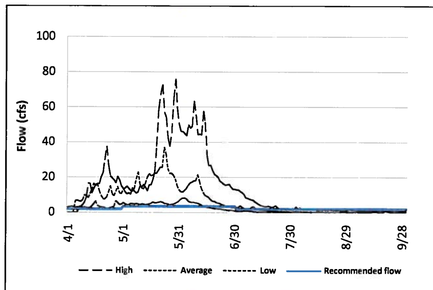
FIGURE 9. Recommended instream flows in Muddy Creek relative to high, average and dry water years for times of year when gage data are available (April through September).
