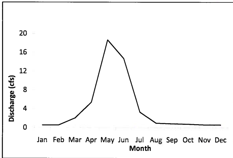
FIGURE 5. Estimated mean monthly flow in Muddy Creek for the period of record. Flow in October through March is estimated.
