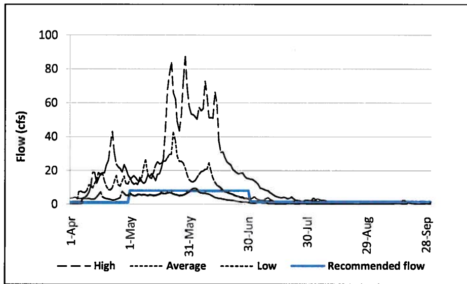
FIGURE 27. Recommended instream flows in McKinney Creek relative to high, average and low flow years for times of year when gage data are available (April through September).
