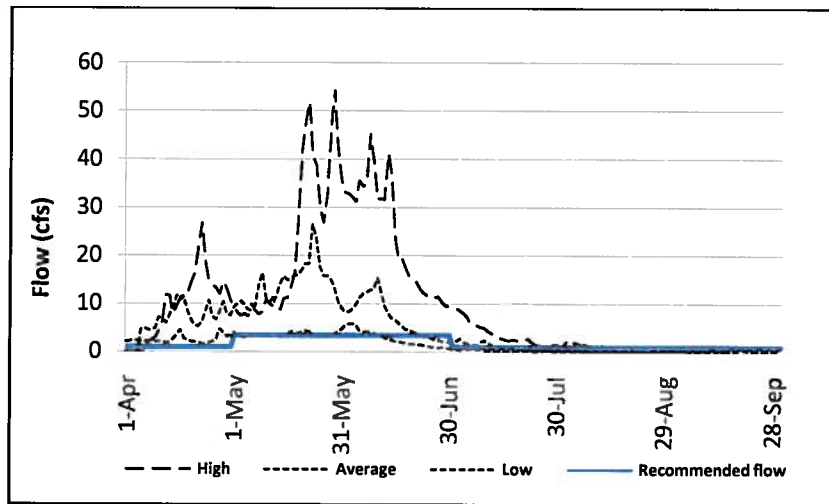
FIGURE 15. Recommended instream flows in Littlefield Creek relative to high, average, and dry water years for times of year when gage data are available (April through September).
