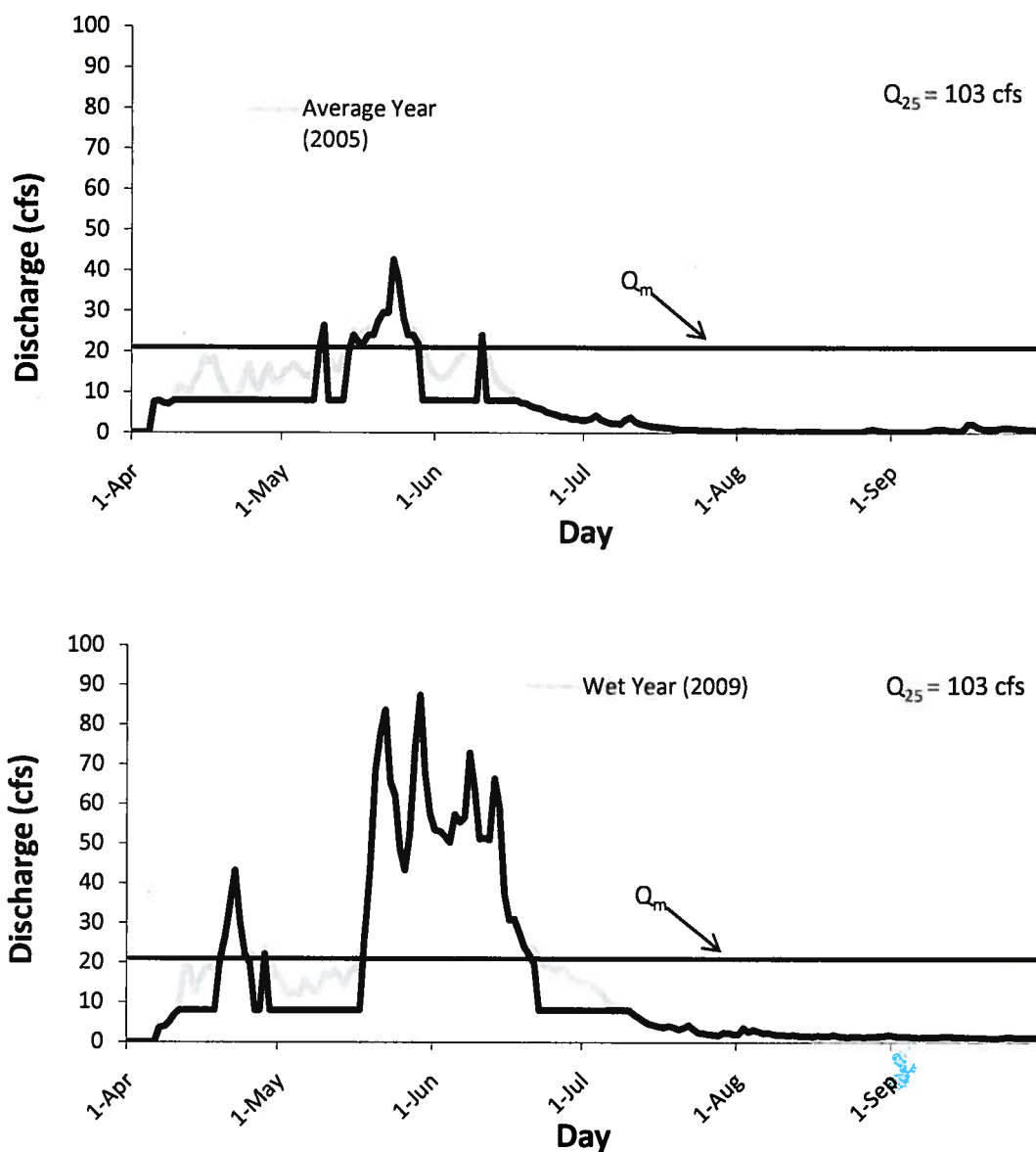
FIGURE A-6. Channel maintenance flow recommendations and hydrographs for the McKinney Creek instream flow segment in an average (2005) and a wet (2009) water year.
