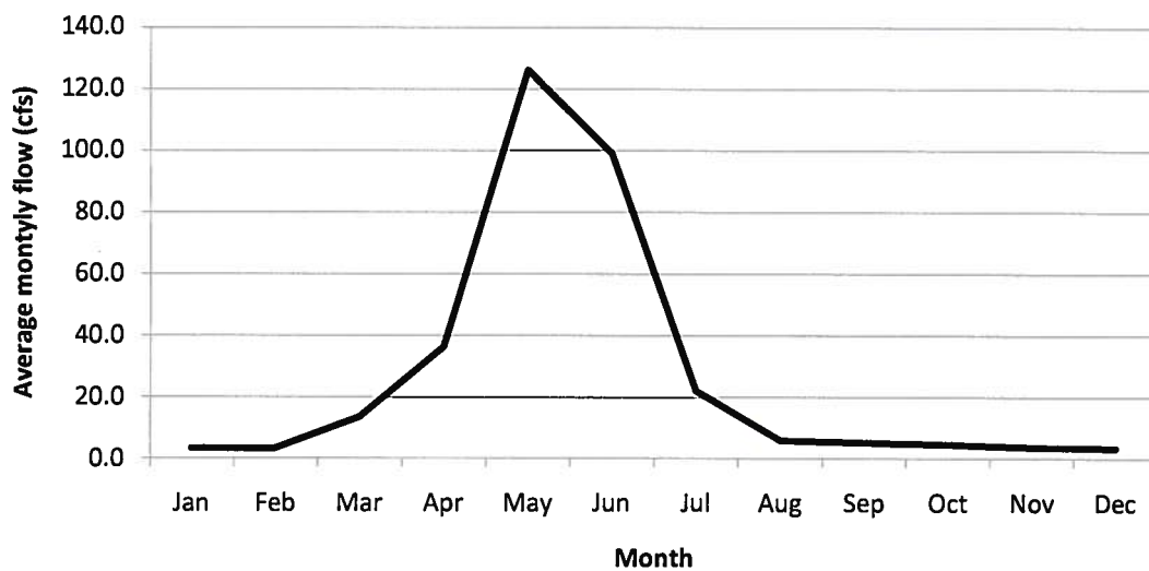
FIGURE 2. Average monthly flow at Jack Creek (USGS stream gage 06627800) from 1990 to 2010. Flows from October through February were estimated by assuming 80% of average September flow. March flows were interpolated based on April and September flows.
