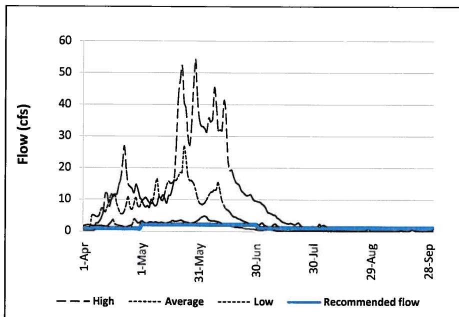
FIGURE 21. Recommended instream flows in Little Muddy Creek relative to high, average, and low flow years for times of year when gage data are available (April through September).
