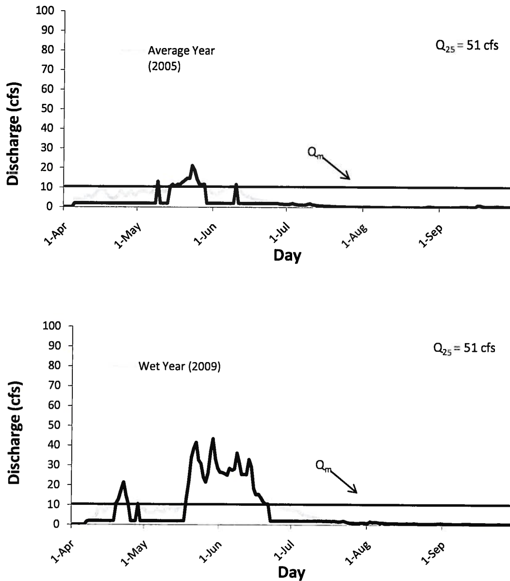
FIGURE A-4. Channel maintenance flow recommendations and hydrographs for the Little Muddy Creek instream flow segment in an average (2005) and a wet (2009) water year.
