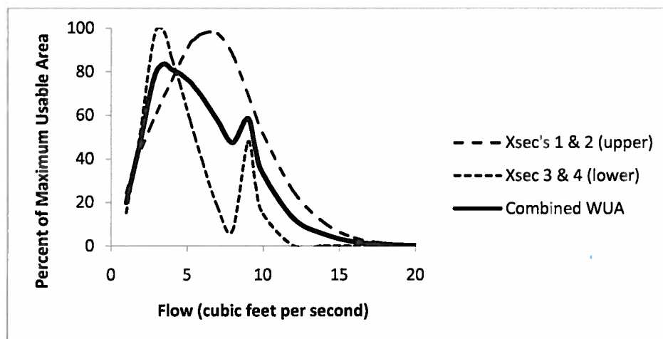
FIGURE 7. Weighted usable area available for CRC spawning at two study sites in Muddy Creek over a range of flows.
