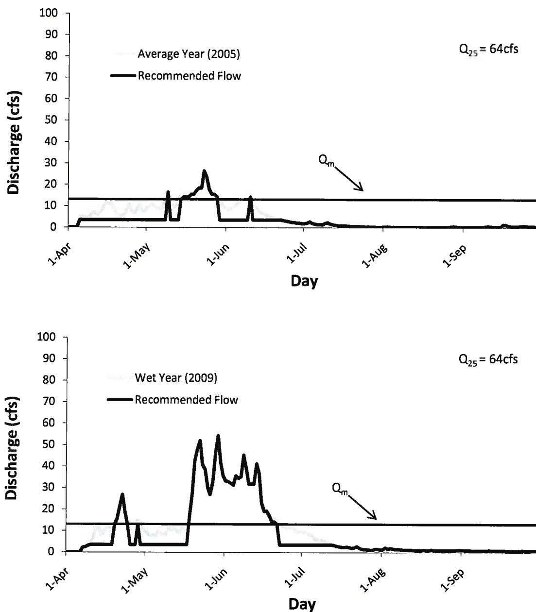
FIGURE A-5. Channel maintenance flow recommendations and hydrographs for the Littlefield Creek instream flow segment in an average (2005) and a wet (2009) water year.
