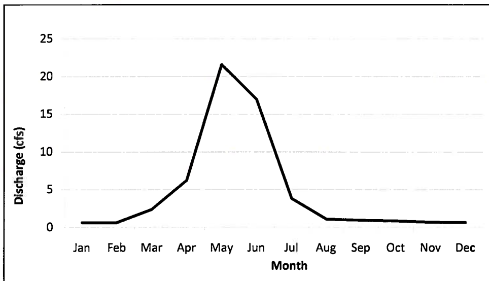
FIGURE 23. Estimated mean monthly flow in McKinney Creek for the period of record. Flow in October through March is estimated.
