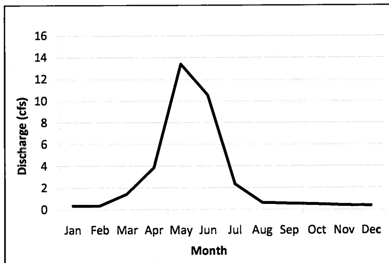
FIGURE 11. Estimated mean monthly flow in Littlefield Creek for the period of record. Flow in October through March is estimated.
