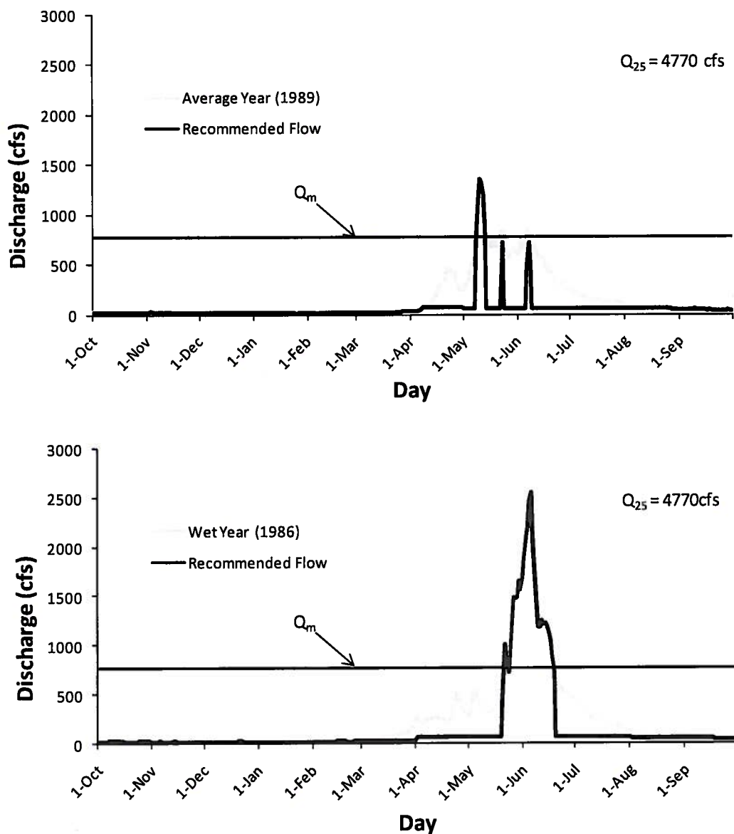
FIGURE B-3. Channel maintenance flow recommendations and hydrographs for the Granite Creek instream flow segment in an average (1989) and a wet (1986) water year.
