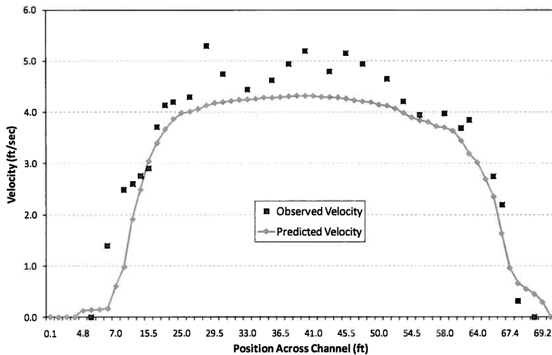
FIGURE 8. Final model-predicted and observed velocities at 399 cfs along the upstream cross-section in the Granite Creek study site.
