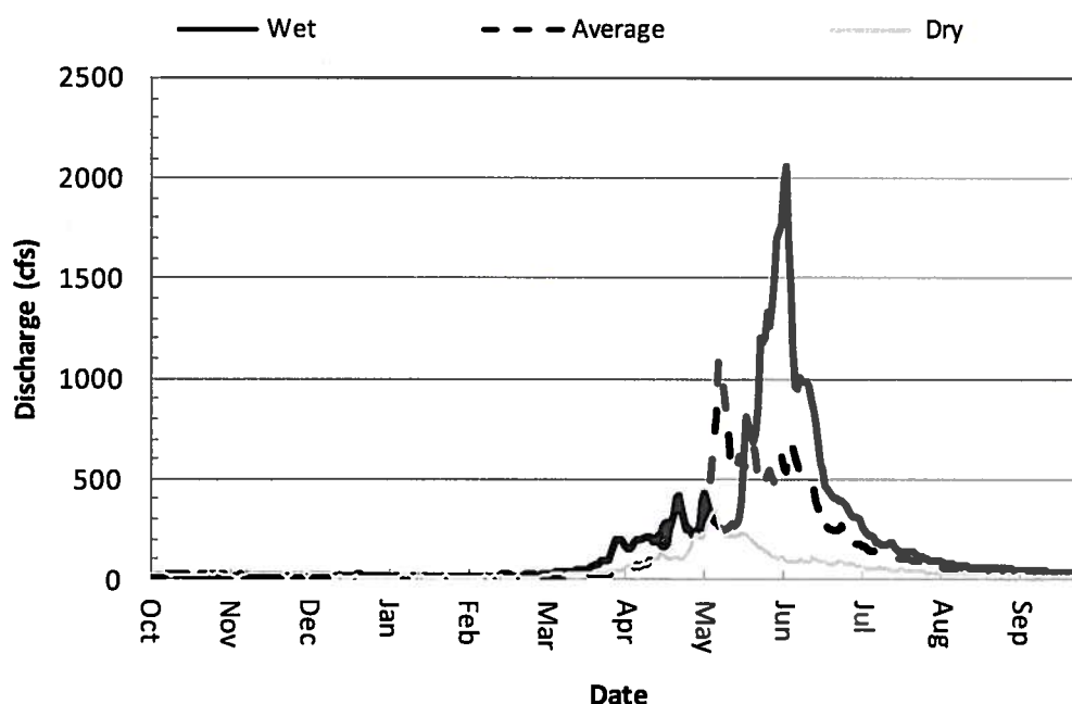
FIGURE 5. Simulated annual hydrographs for wet, dry, and average conditions at the Granite Creek instream flow segment (HabiTech 2009).
