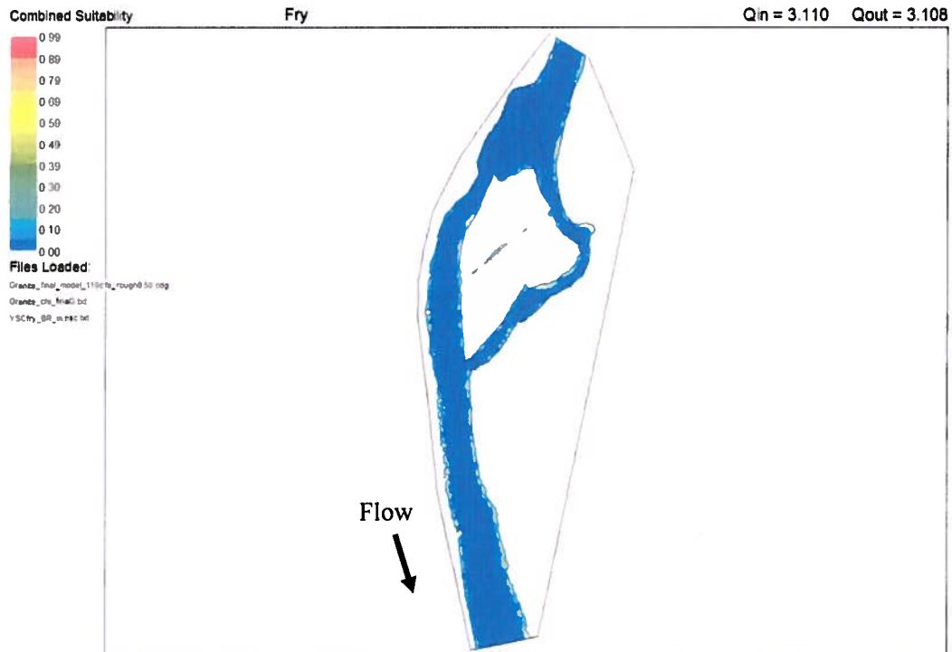
FIGURE 10. Combined suitability for SRC fry in the Granite Creek study site at 110 cfs discharge.
