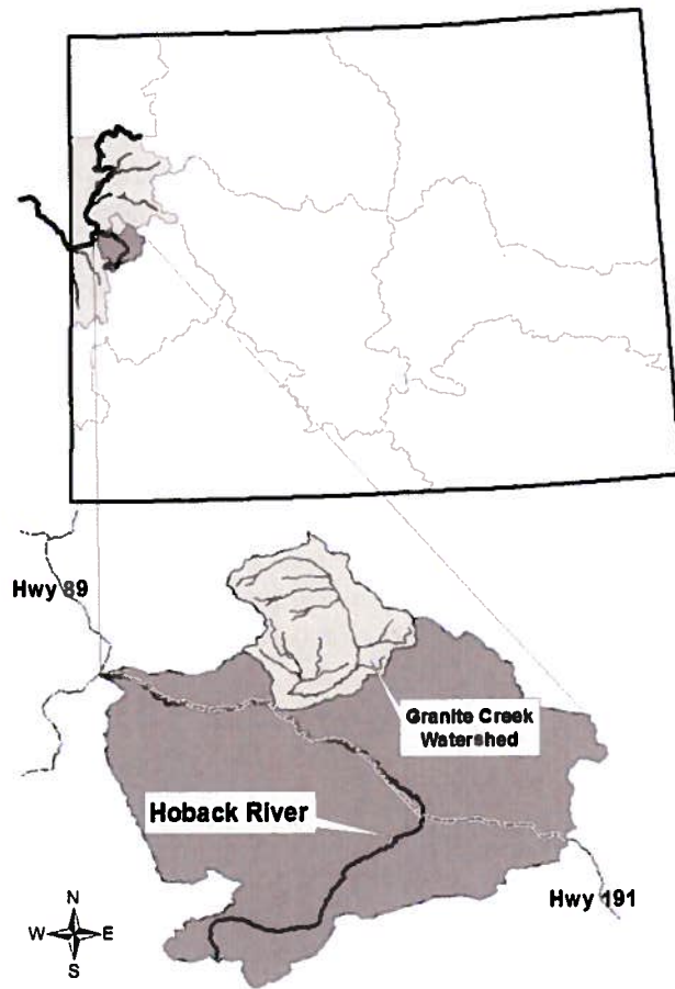
FIGURE 1. Location of Granite Creek, Wyoming (HUC 170401030405) in the Hoback River watershed.
