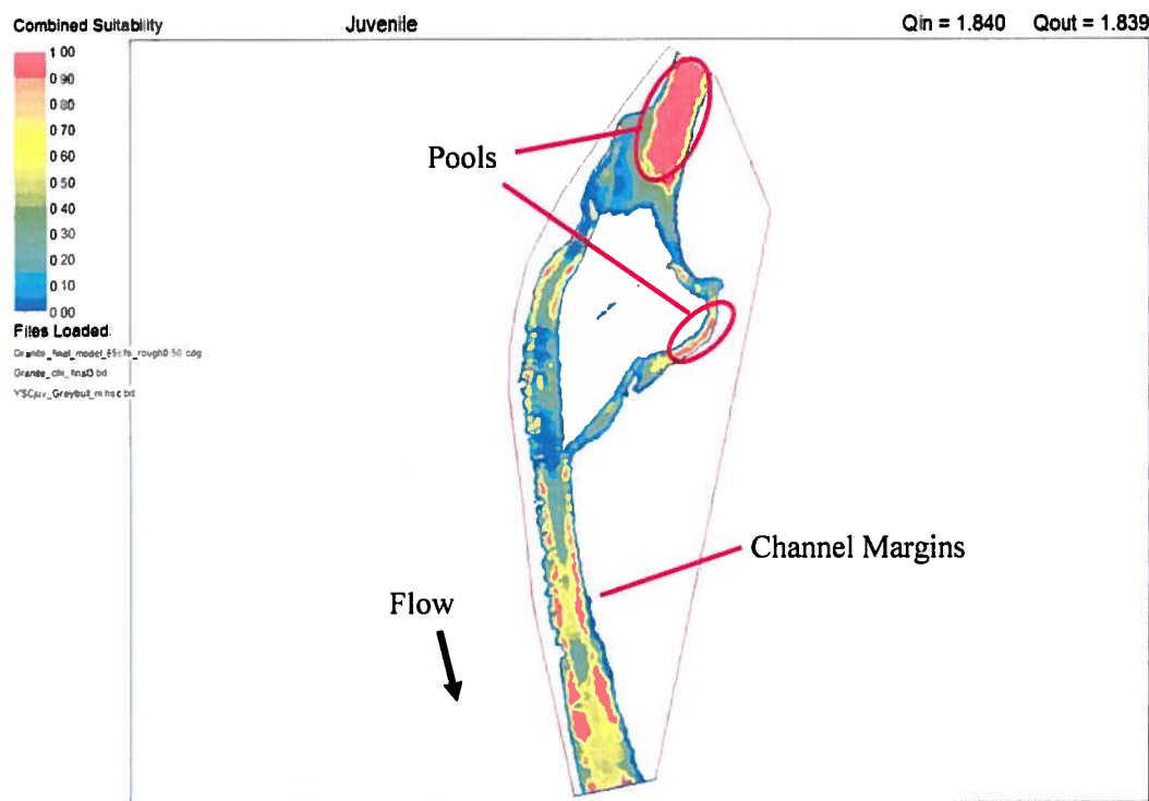
FIGURE 11. Combined suitability for juvenile SRC in the Granite Creek study site at 65 cfs discharge.
