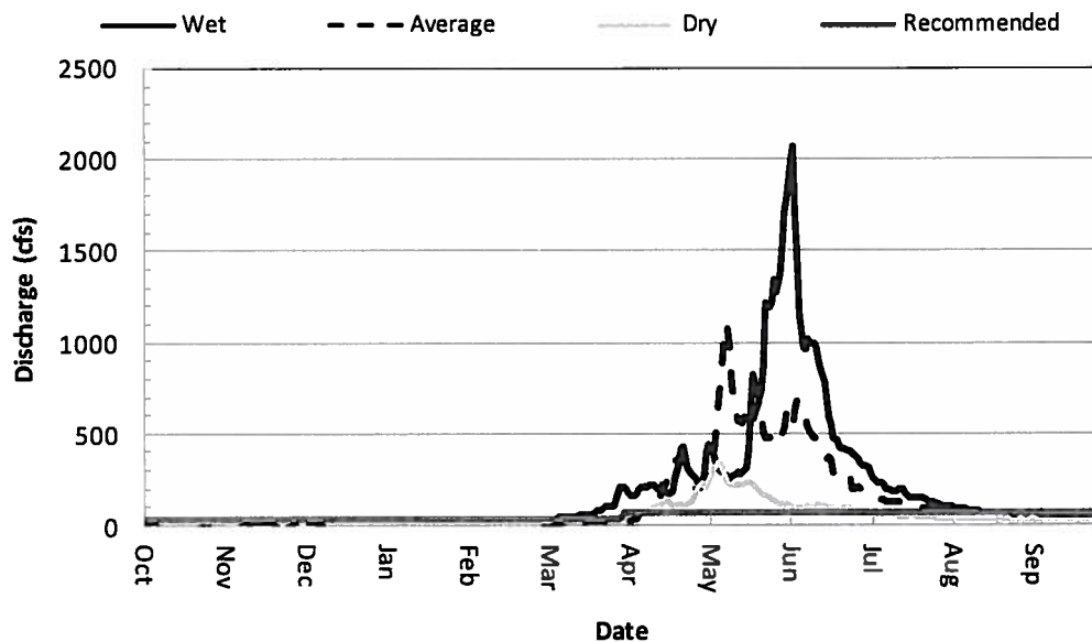
FIGURE 15. Recommended instream flows in the proposed segment (when available) relative to wet, dry, and average flow years.
