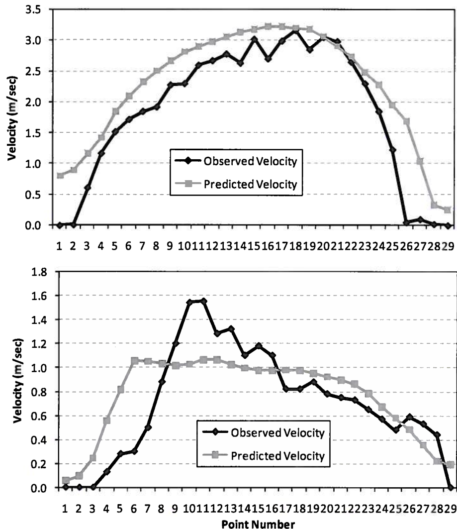
FIGURE 7. Final model-predicted and observed velocities at 141 cfs along the two side channel cross-sections in the Granite Creek study site.
