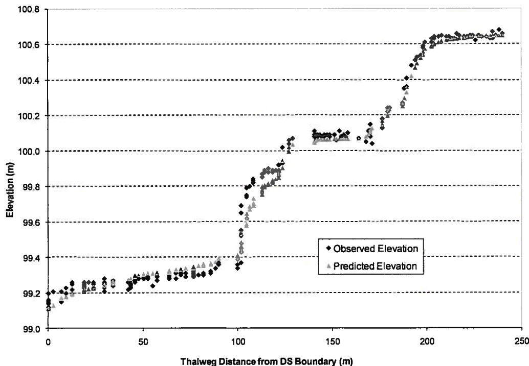
FIGURE 6. Final model-predicted and observed water surface elevations at 74 cfs along the right bank in the Granite Creek study site.
