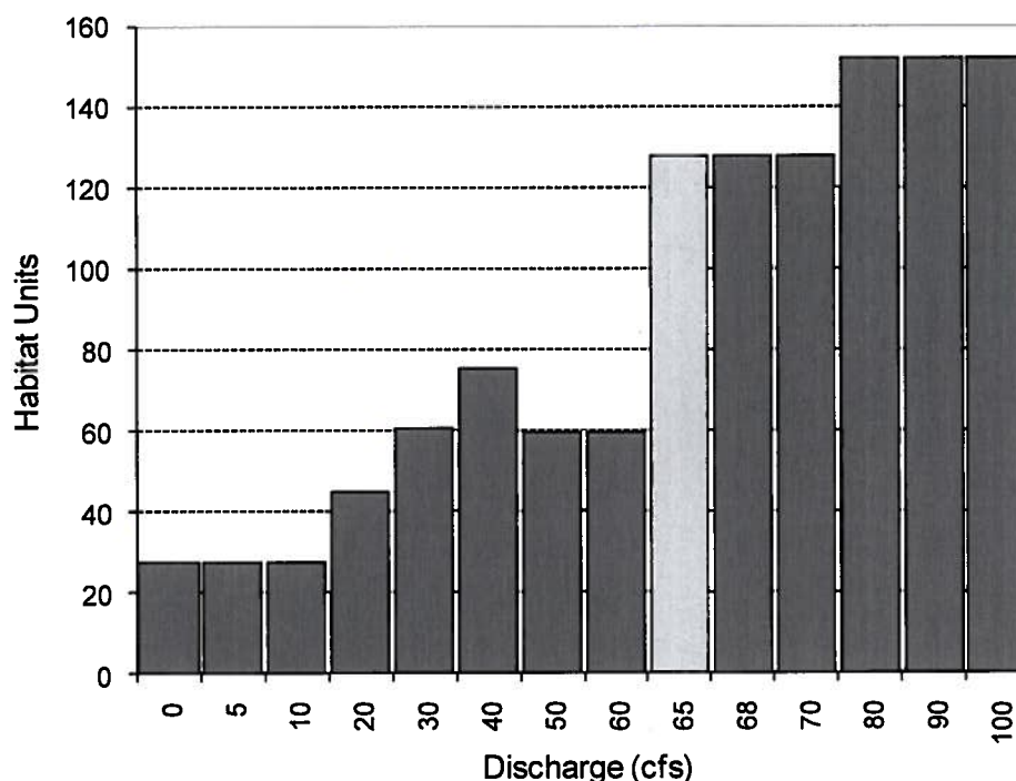
FIGURE 14. Habitat Quality Index vs. discharge in the Granite Creek instream flow segment. X-axis values are not to scale; the values were chosen to indicate where changes in Habitat Units occur. The recommended flow is indicated by the light shaded bar.
